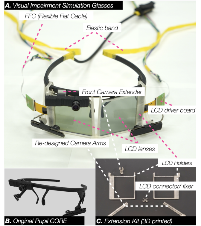
Figure 2: A. depicts the assembled Visual Impairment Simulation Glasses with two extra elastic bands to fasten the device to the user’s head minimizing undesired displacement. B. indicates the original Pupil CORE eye-tracker. C. is the extension kit that we designed and 3D printed for modifying Pupil CORE into Real-time Visual Impaired Effects Rendering Glasses.
